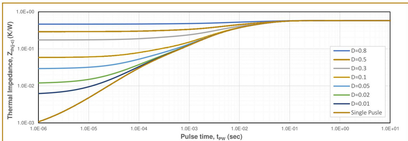
Fig.21 Transient Junction to Case Thermal Impedance
