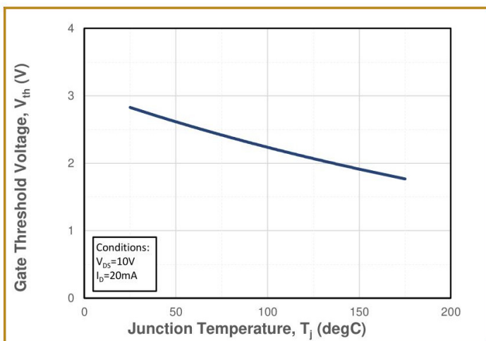
Fig.11 Threshold Voltage vs. Temperature
