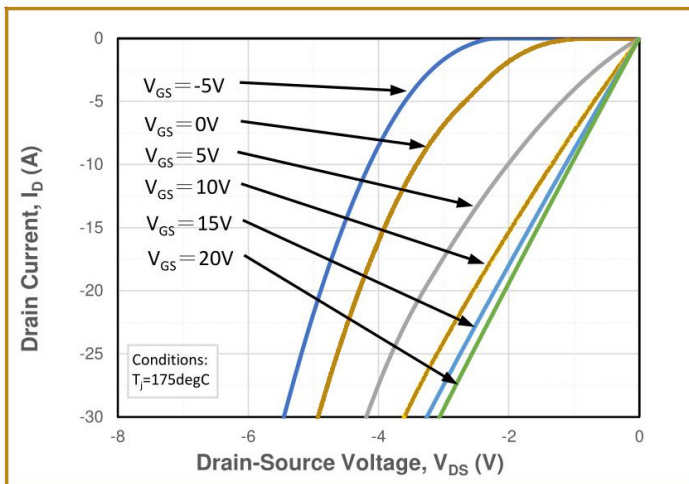
Fig.9 Reverse Output Characteristics at T_J = 175^\circ C
