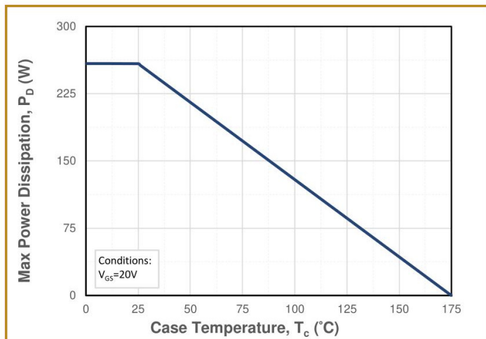
Fig.13 Maximum Power Dissipation Derating vs. Case Temperature
