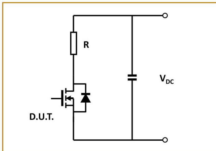
Fig.19 Schematic of Resistive Switching
