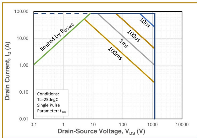
Fig.15 Safe Operating Area
