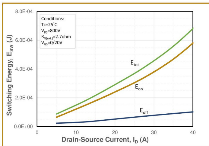
Fig.17 Clamped Inductive Switching Energy vs. Drain Current
