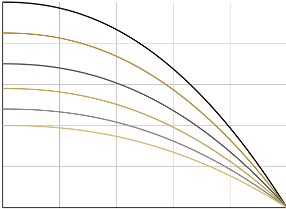
Fig.7 Maximum Forward Current Derating vs. Case Temperature
