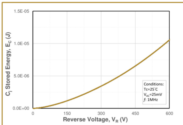
Fig.4 Capacitance Stored Energy
