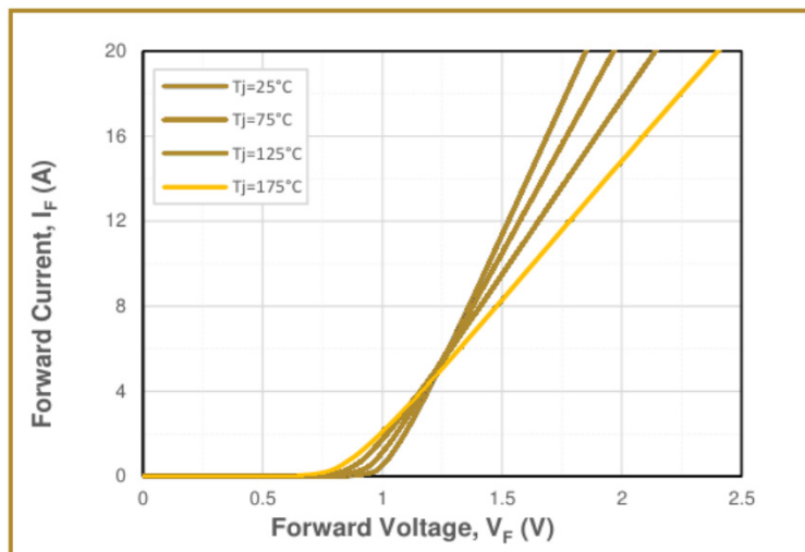
Fig.1 Forward Characteristics
