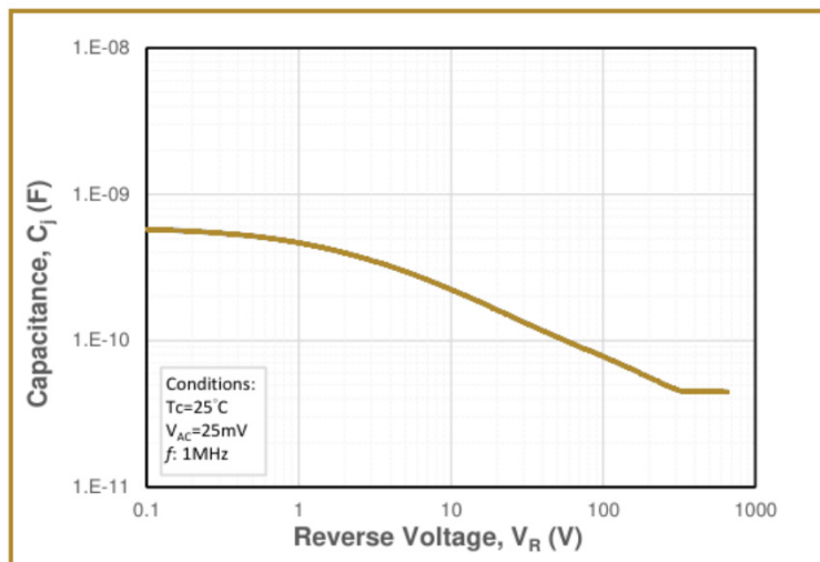
Fig.3 Junction Capacitance vs. Reverse Voltage
