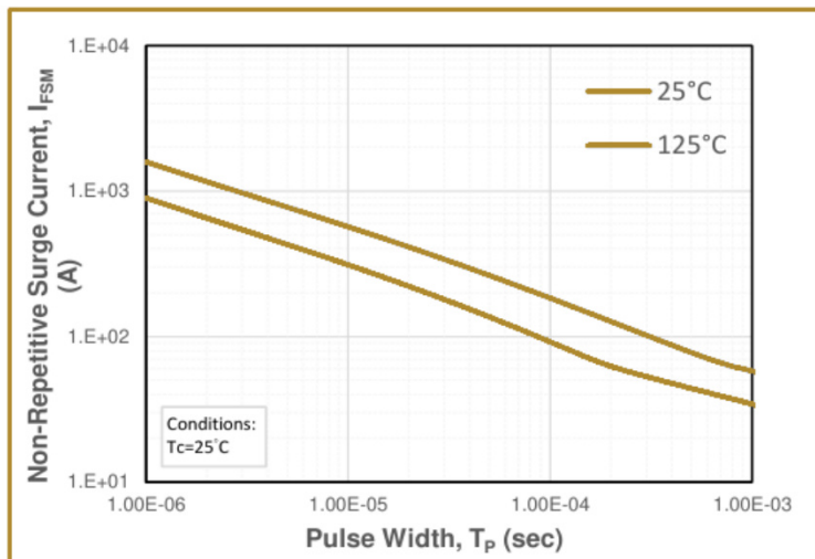
Fig.6 Non-Repetitive Peak Forward Surge Current (Pulse Mode)
