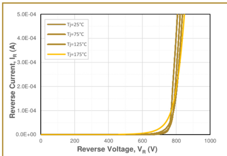
Fig.2 Reverse Characteristics
