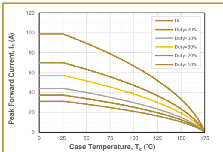
Fig.7 Maximum Forward Current Derating vs. Case Temperature
