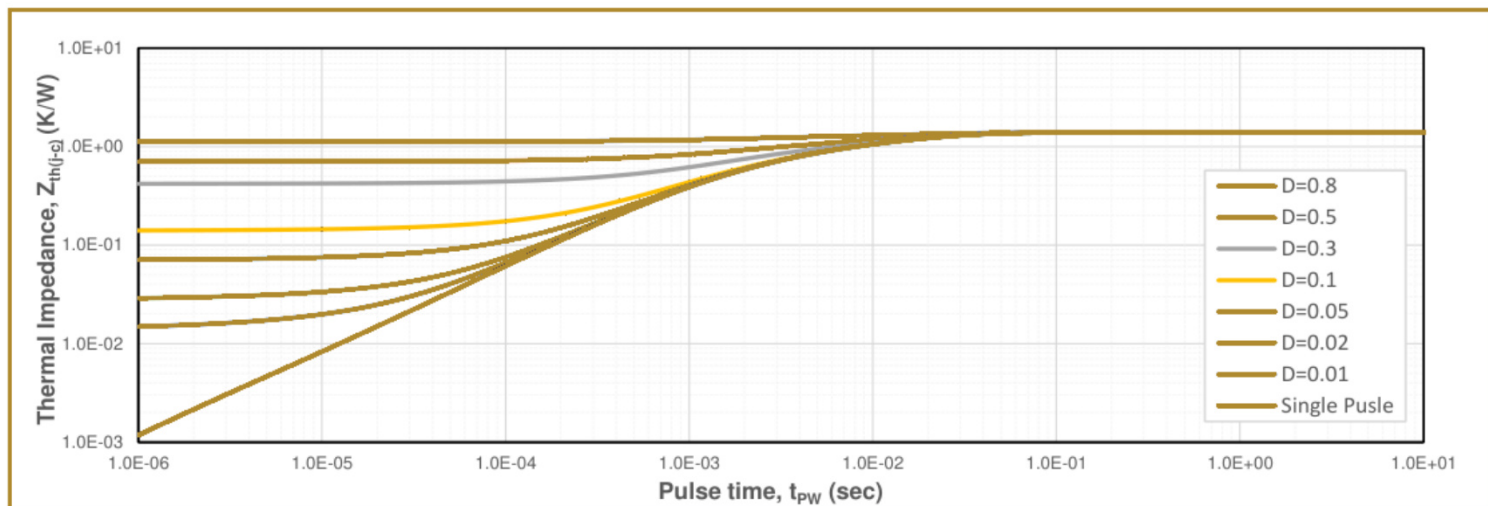
Fig.9 Transient Junction to Case Thermal Impedance
